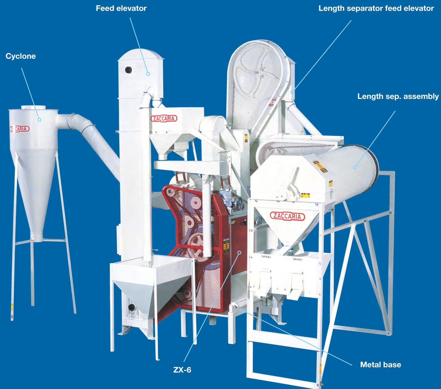
Compact ZX-6 with optional accessories (electric drive)
