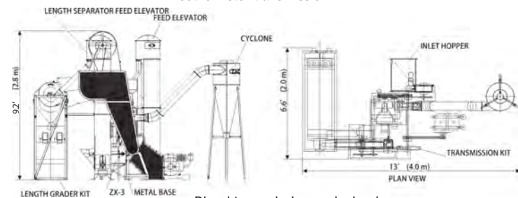
Diesel transmission or single-phase
