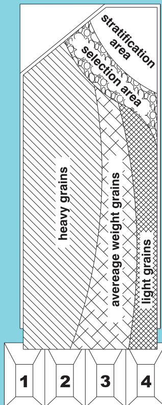
Representative drawing of the machine with right output.
